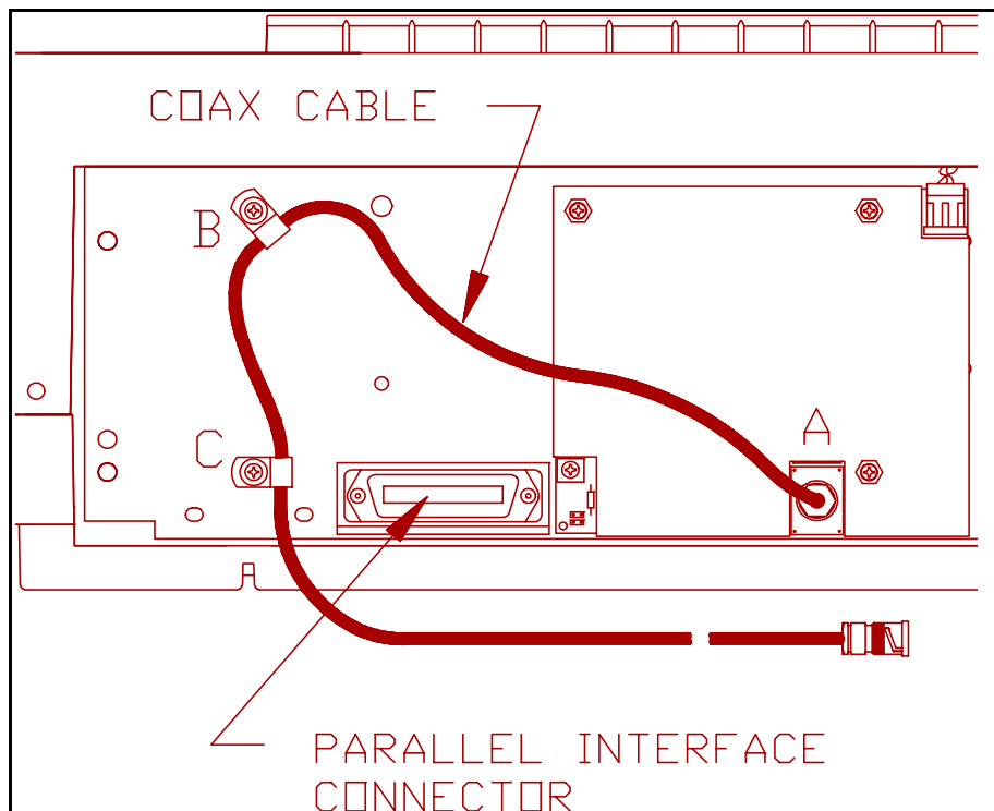
Rear View of Printer
